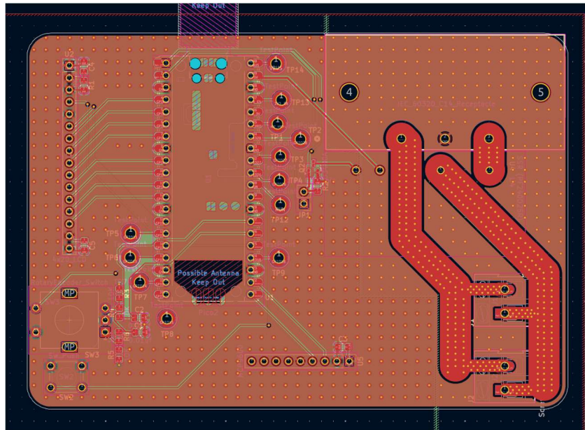
Figure 11: Routed PCB, Maiorov 2026
