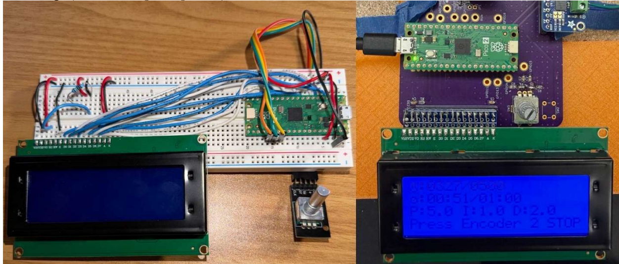
Figure 9: HMI prototype (Left) Final (Right), Maiorov 2026
