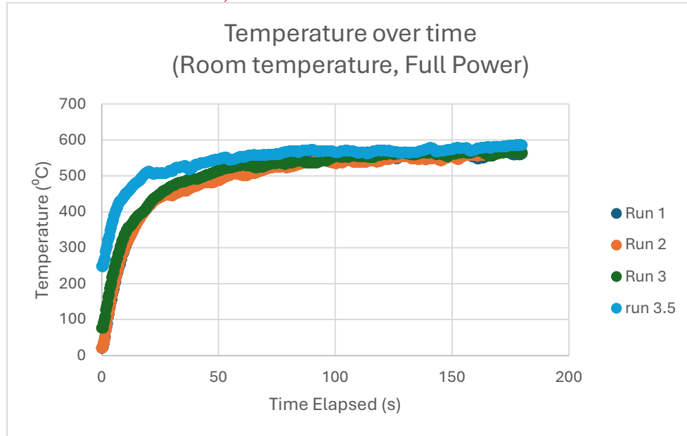
Figure 15: Max Temperature Test, Maiorov 2026
