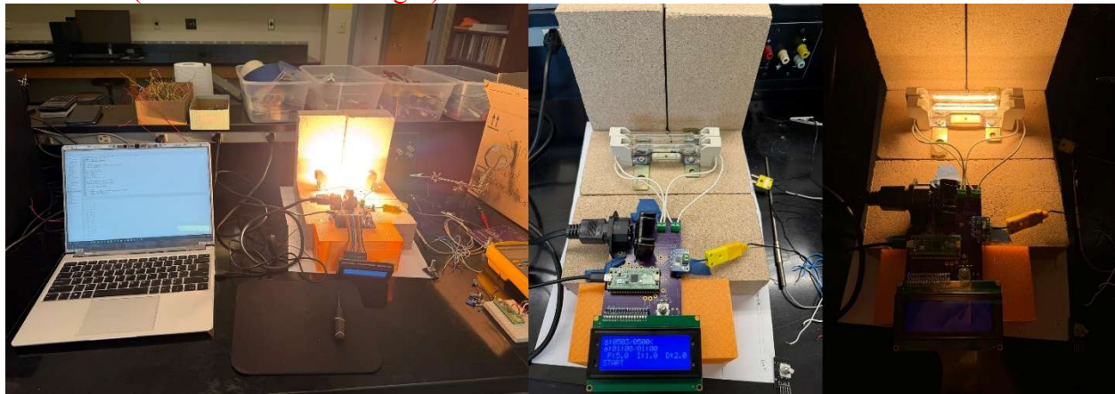
Figure 17: Computer connected Oven (left), Final Oven (OFF) (center), Final Oven (ON) (right), Maiorov 2026
