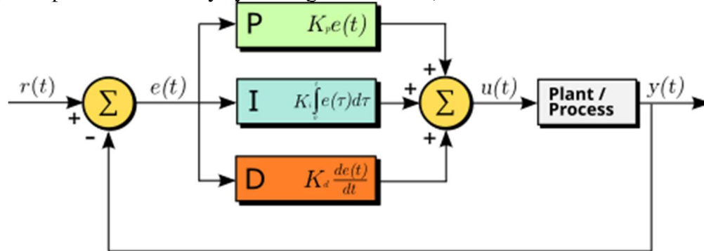
Figure 12: Wikipedia 2026, “Proportional–integral–derivative controller”
