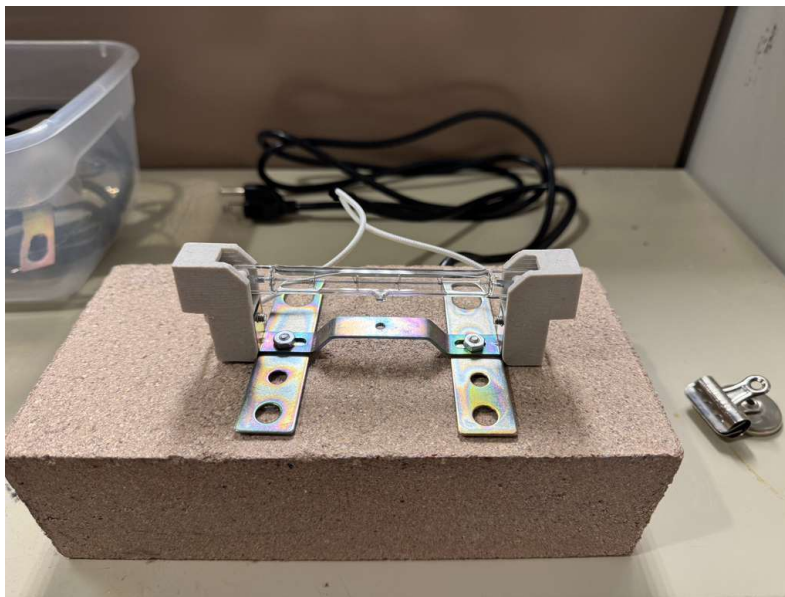
Figure 1: Current oven setup, Maiorov 2025
