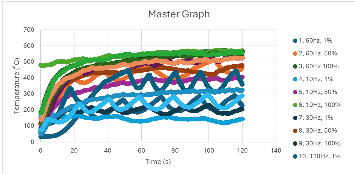
Figure 14: PWM tests at varying frequencies and Duty cycles, Maiores 2026
