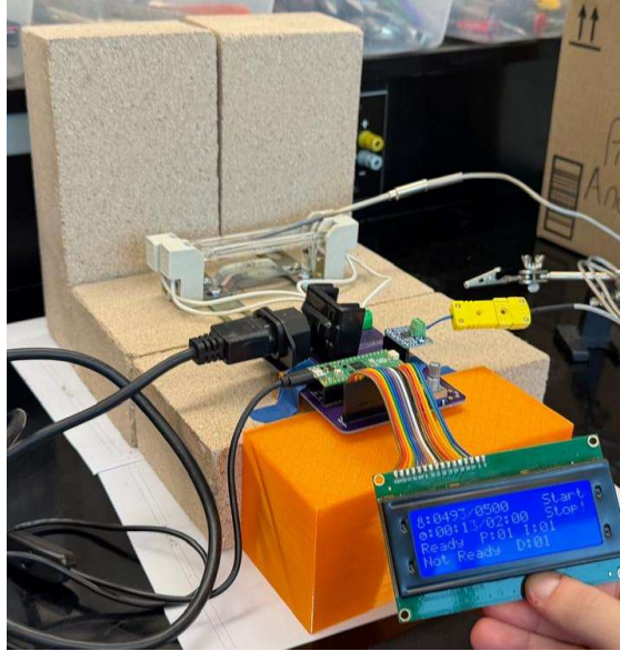
Figure 13: Initial Prototype, Maiores 2026
