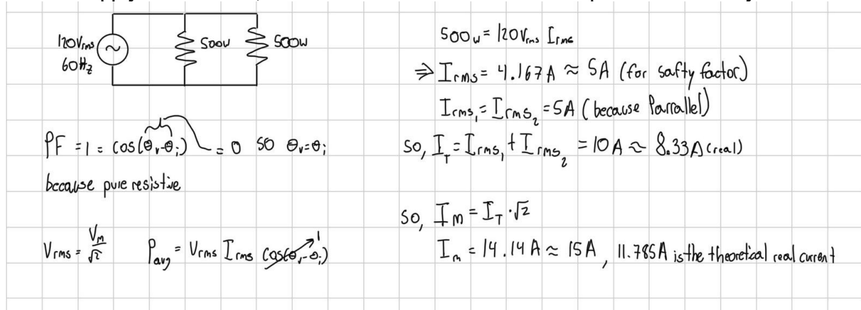
Figure 10: Circuit Analysis, Maiorov 2026)
